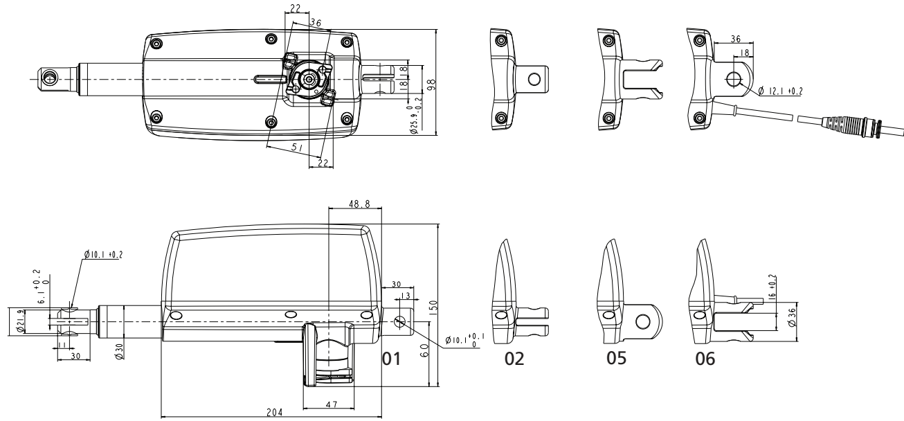
Drawing no.: LA32F001C
