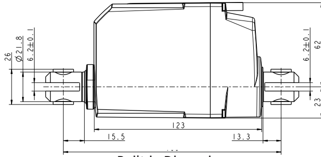
Built-in Dimensions
