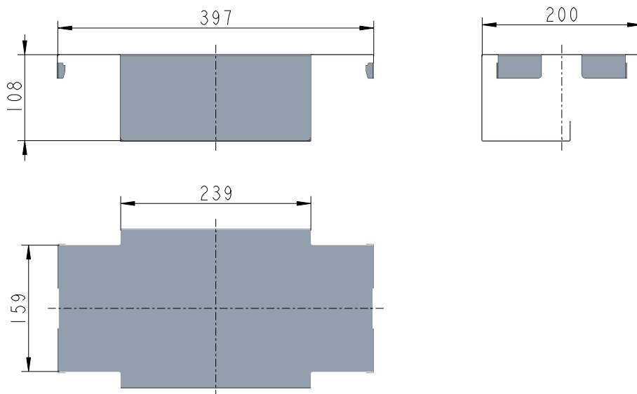
Bridge dimensions (mm)
