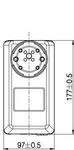
Motor housing
