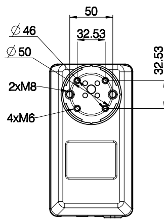
Bottom plate
