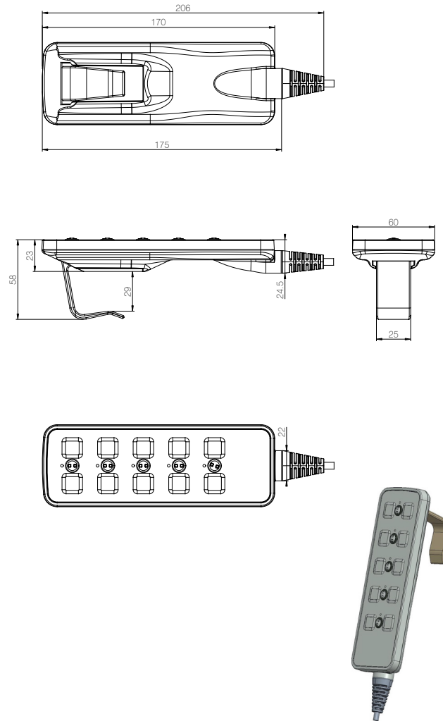
HL400 with Hook type 2
