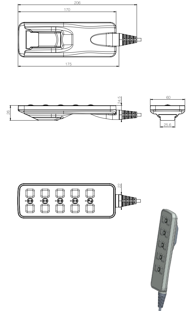
HL400 with magnet (Hook type 1)
