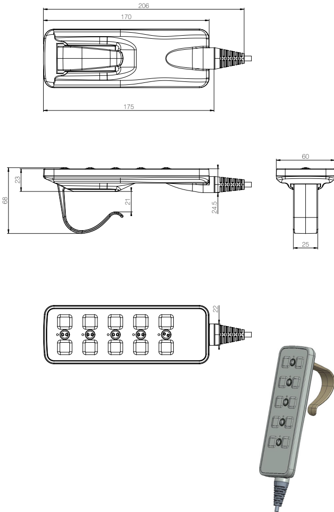
HL400 with Hook type 0
