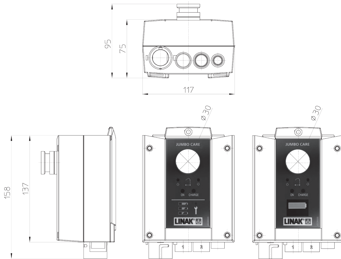
Drawing no.:CBJ001C
