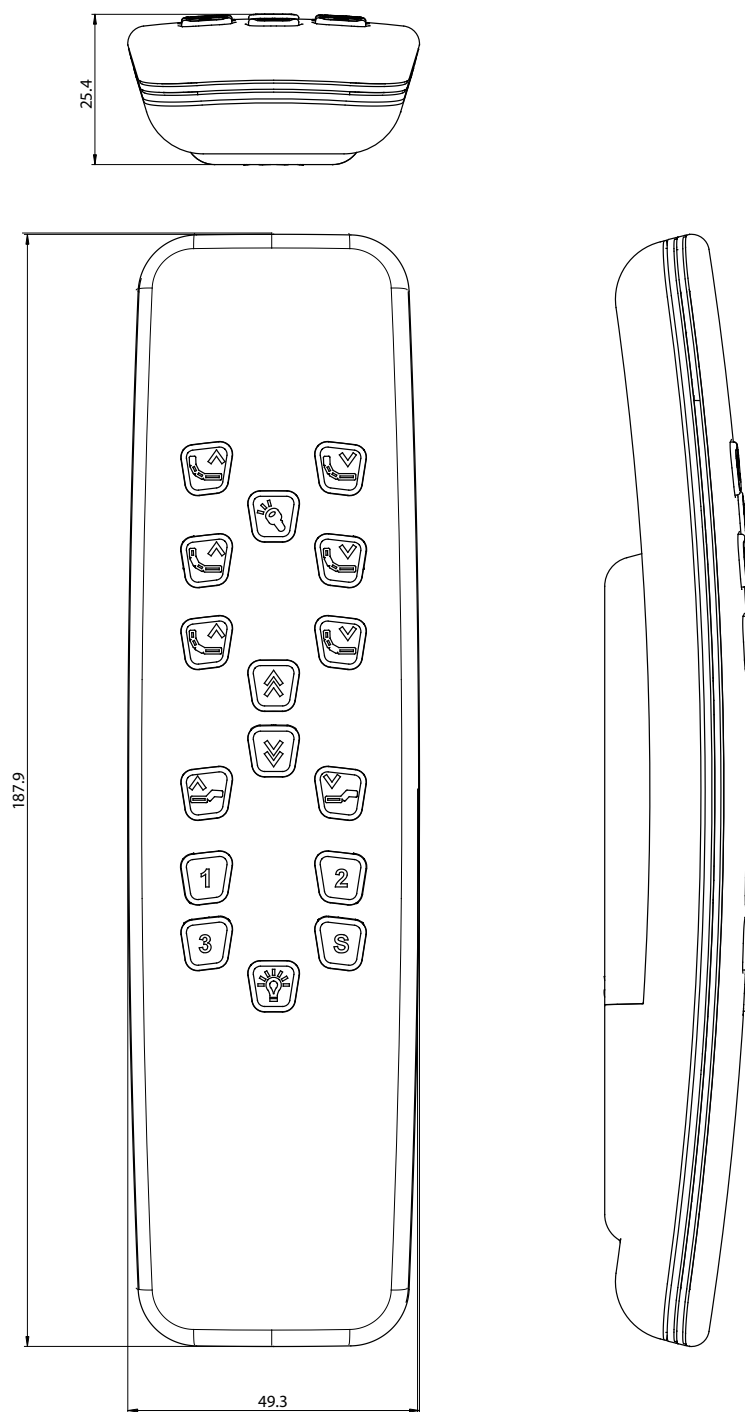
Figure 1 Hc20 dimensions (mm)
