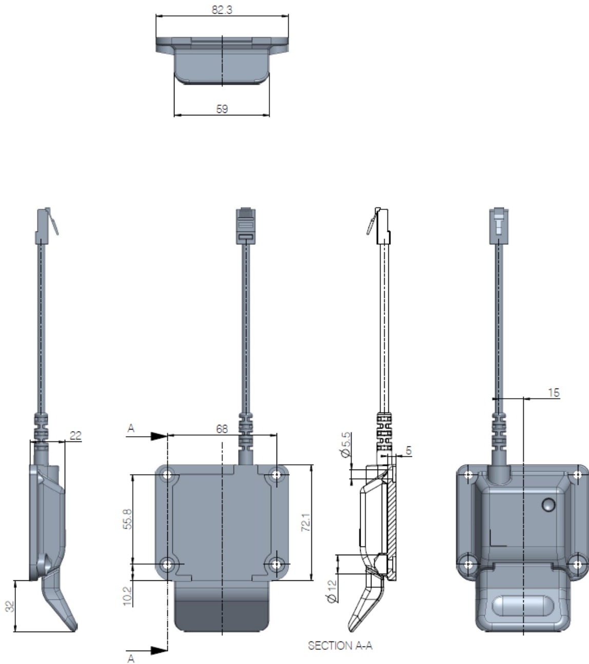
Figure 1 DPI1C dimensions (mm)
