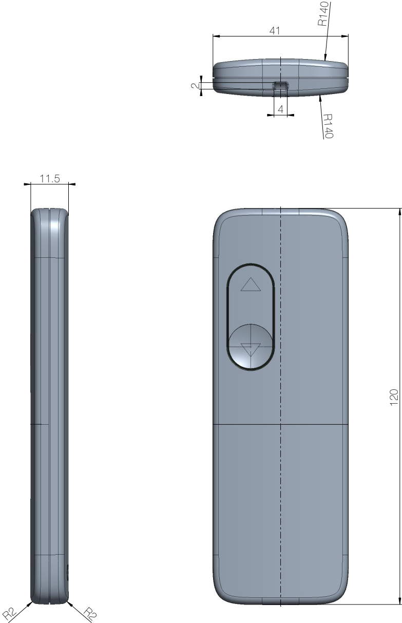
Figure 1 BP11 TV dimensions (mm)
