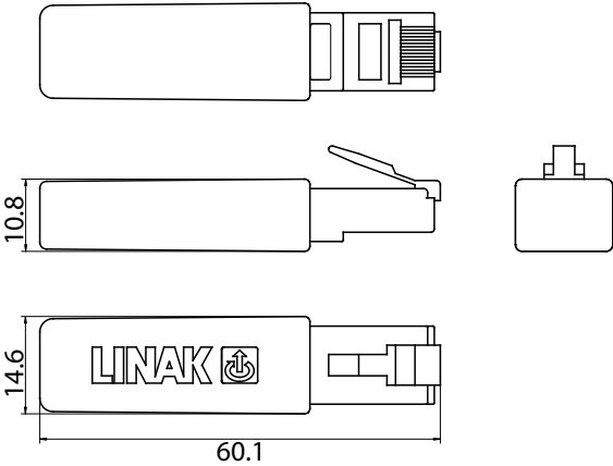
DS2 dimensions (mm)
