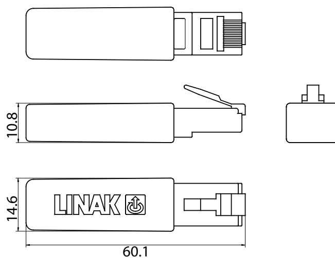
Figure 1 Bluetooth® adapter
